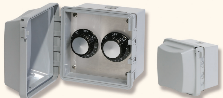
Part # 14-4125 (120V) - Part # 14-4225 (240V) Double Surface Mount w/Weatherproof Box (Includes Two (2) INF Input Regulators)
